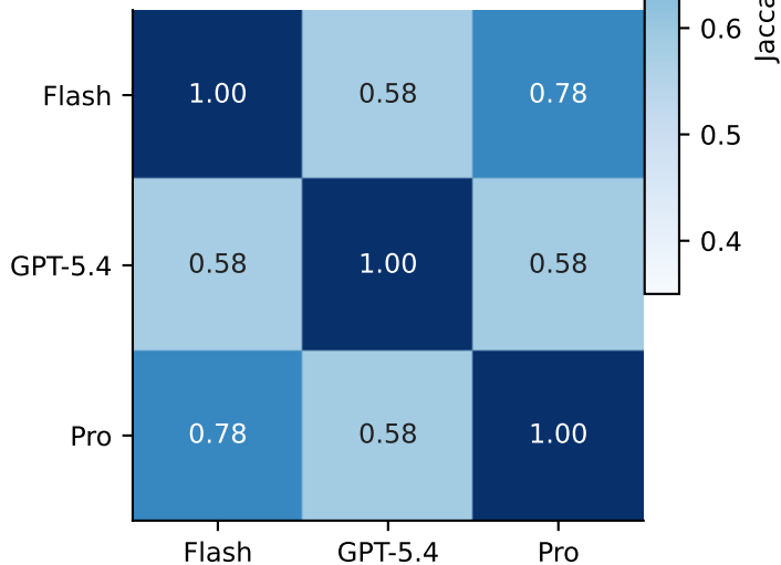
WEBSHOP - Tower
