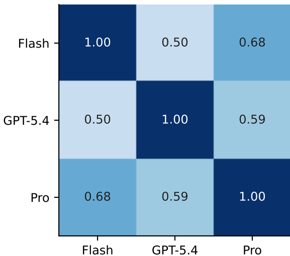
WEBSHOP - No-Skill
