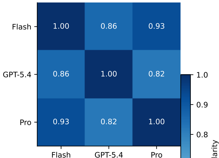
ALFWORLD - Tower
