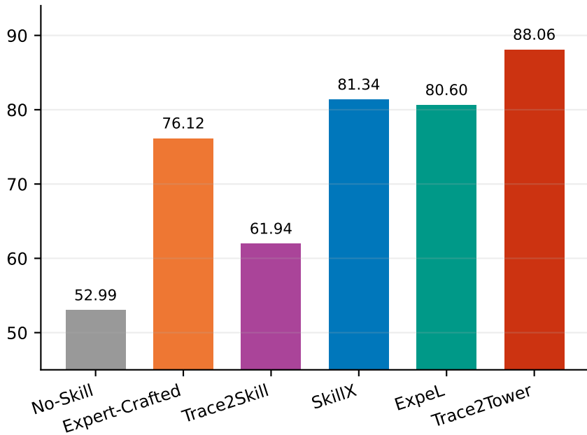
ALFWorld success rate (%)
