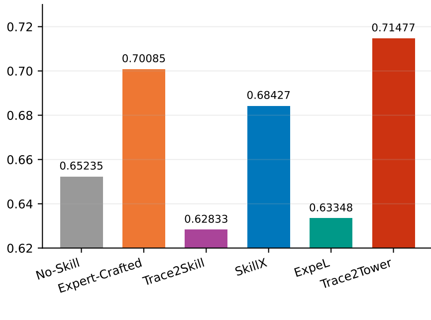
WebShop mean reward
