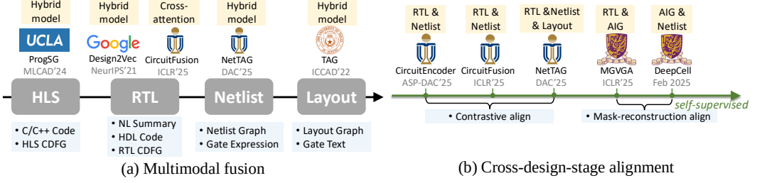
Fig. 10. Timeline for multimodal fused and cross-stage aligned encoders.
