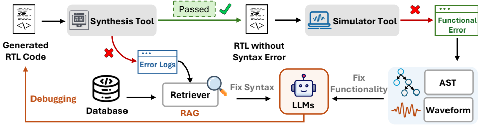
Fig. 18. Overview of the LLM-based flow for RTL debugging, recent works are covered in Section 5.6. This approach includes two input methods for LLM solutions: the first method assigns debugging tasks directly to the LLM without supplementary information, while the second method enhances the debugging process by incorporating error information from EDA tools. This error log can be input directly into the LLM or used to query a pre-defined debugging database (RAG). Additionally, some approaches utilize AST or waveform tracing tools to more effectively identify problematic code segments.
