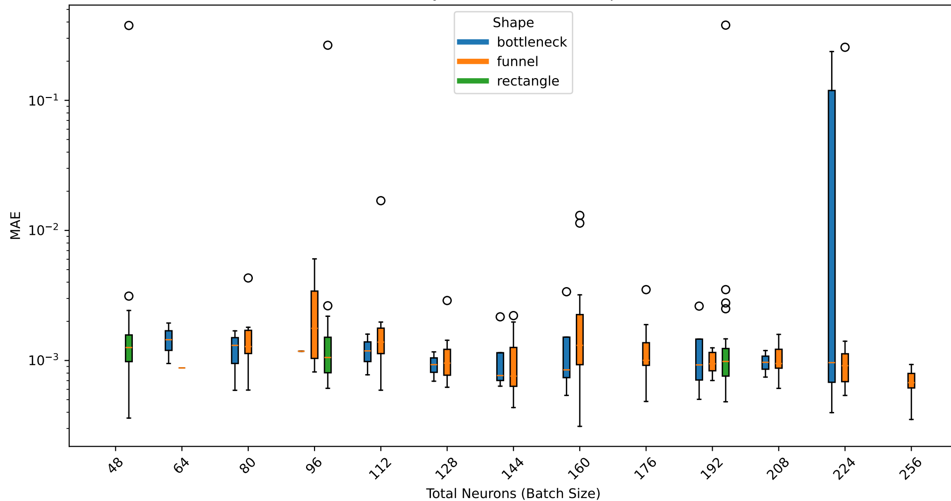
MAE Distribution by Neuron Count & Shape for Problem B
