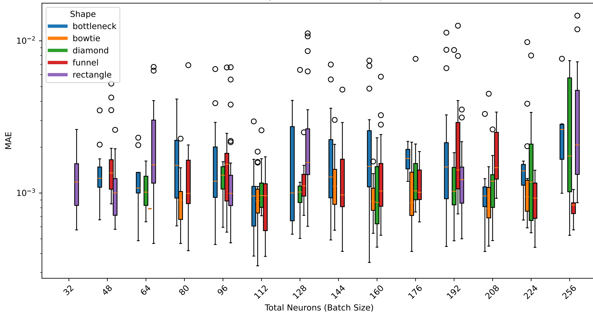
MAE Distribution by Neuron Count & Shape for Problem A
