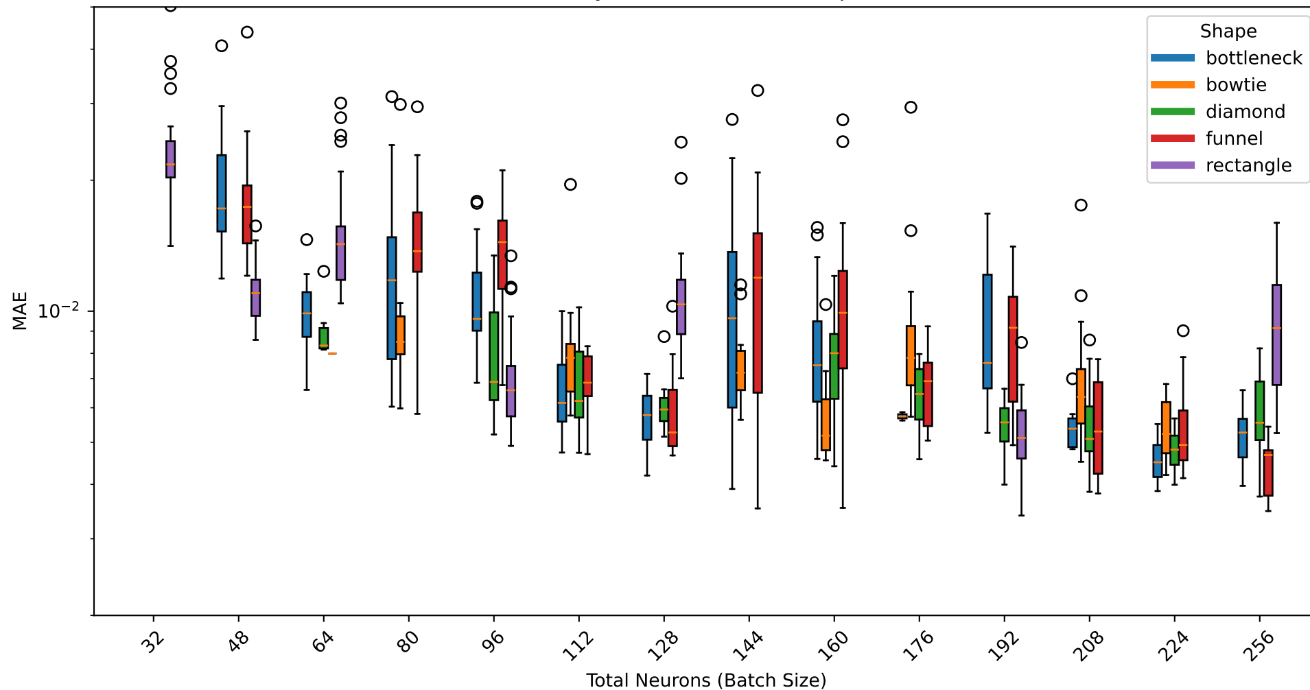
MAE Distribution by Neuron Count & Shape for Problem C
