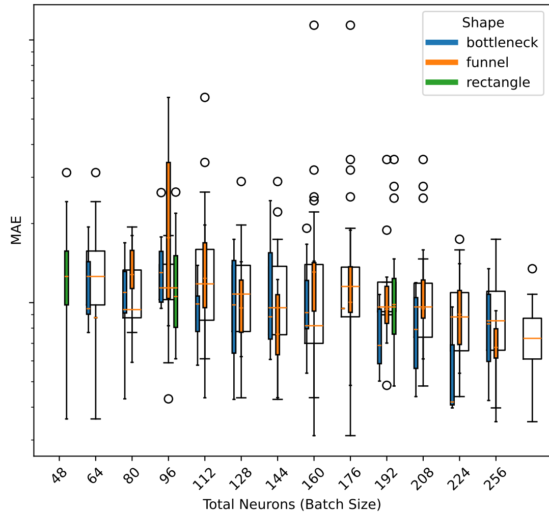
MAE Distribution by Neuron Count &amp; Shape for Problem D
