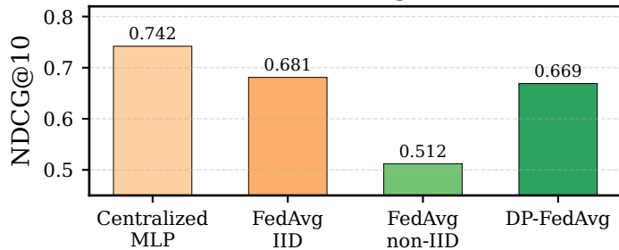
(b) NDCG@10
