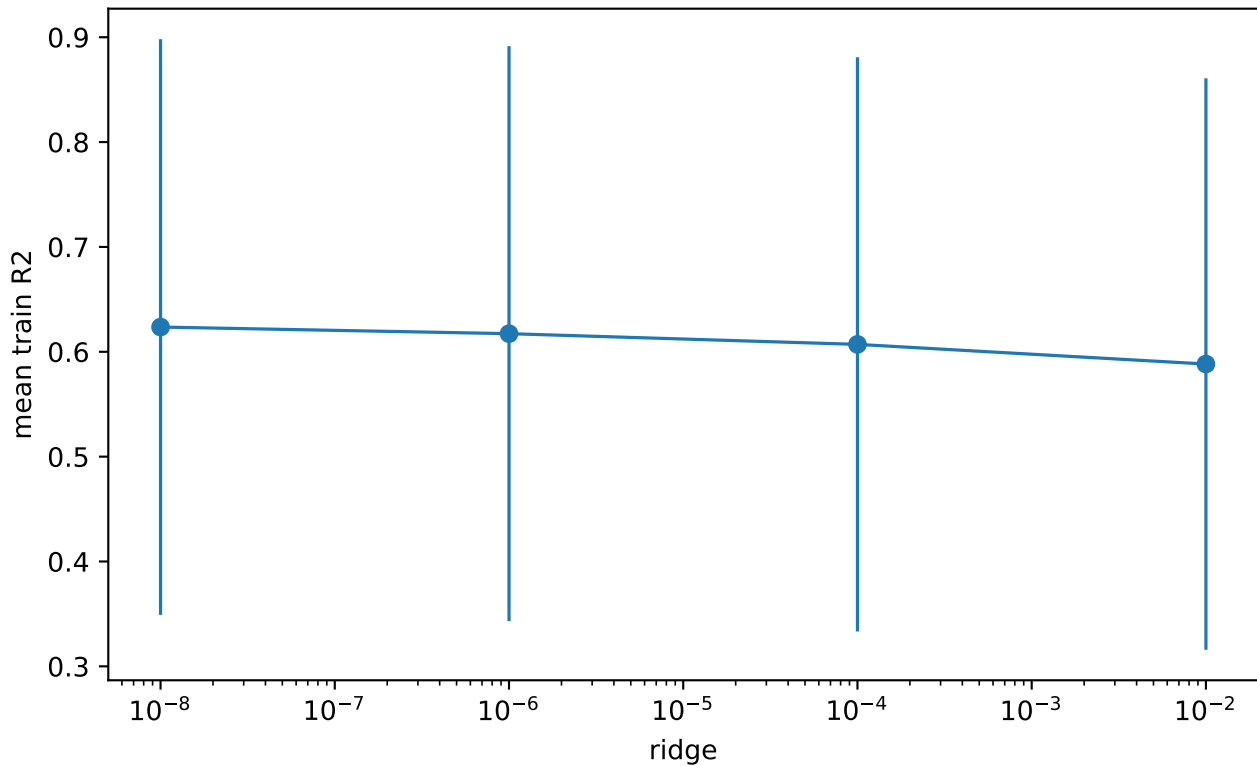
Ridge path summary
