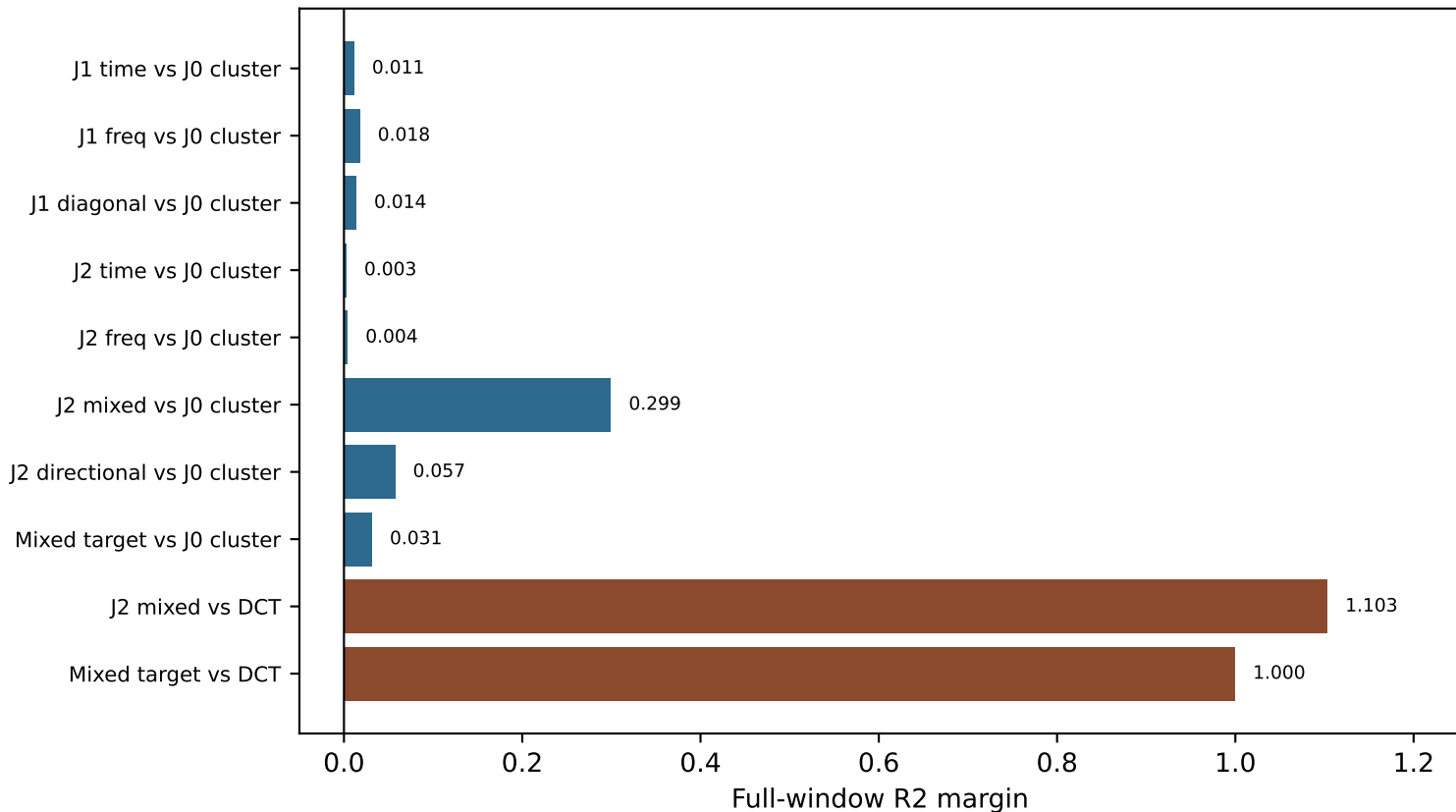
Positive margins for matching high-order PJ spaces
