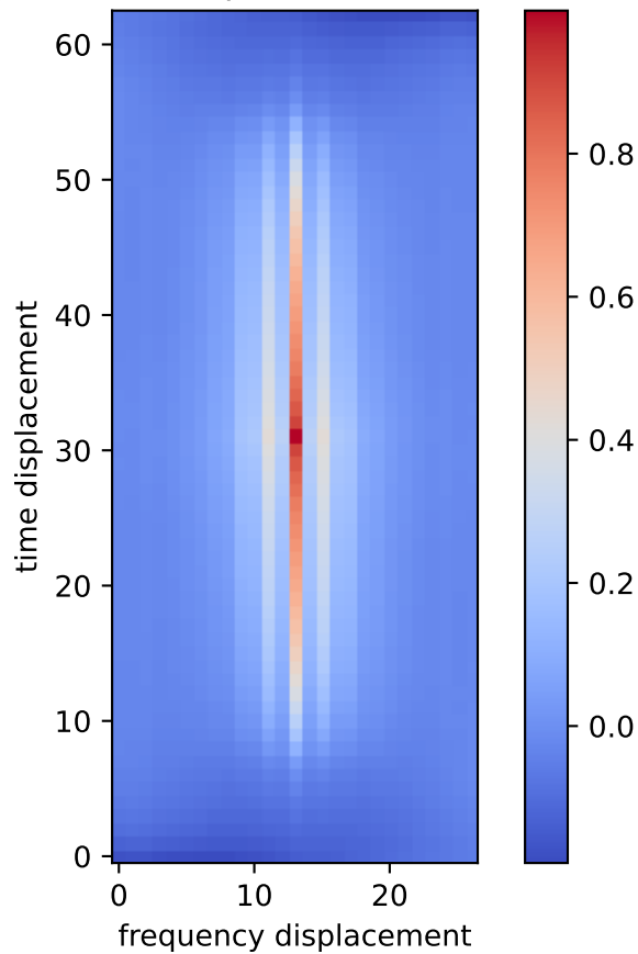
NSynth CQT empirical offset covariance
