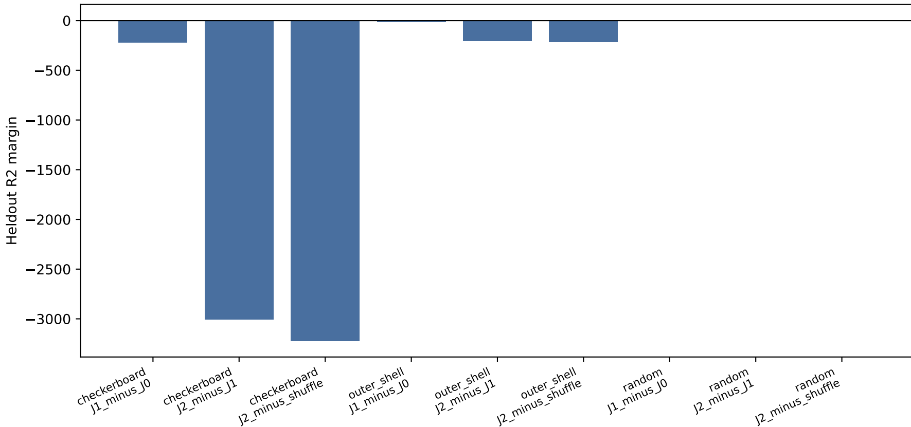
Heldout-offset margins for learned NSynth scalar-bias tables
