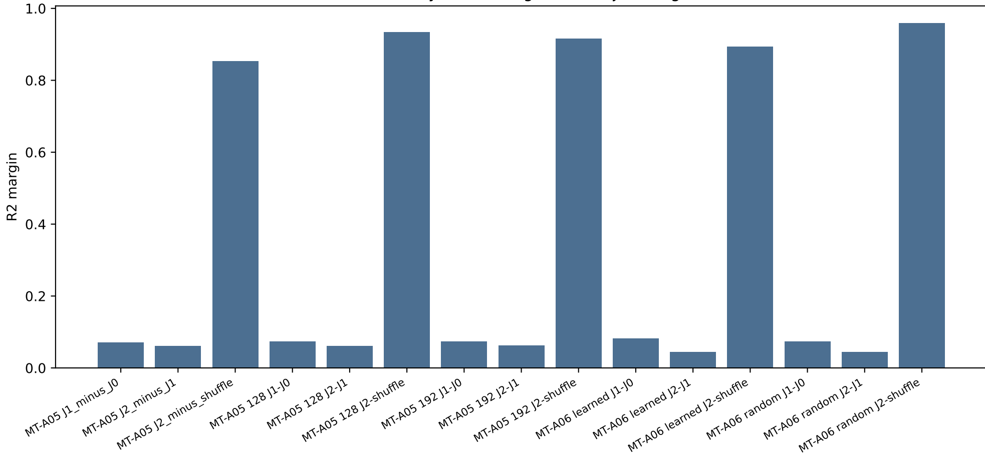
Audited NSynth/CQT higher-order jet margins
