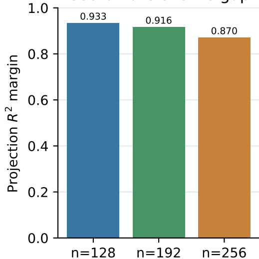
Coordinate-shuffle gap
