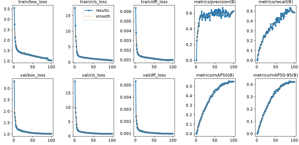
图 8: Stage 2 (YOLO26s-P2) 训练曲线
