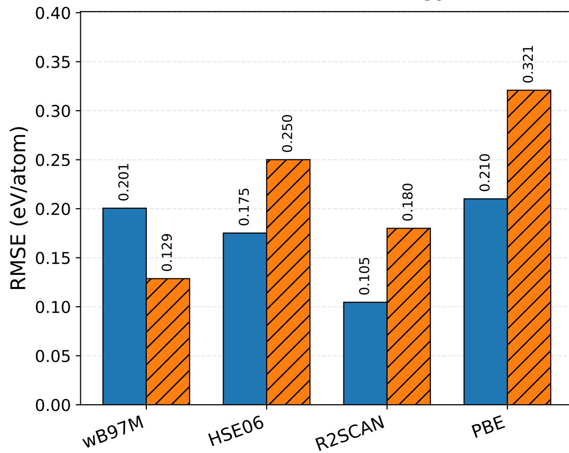
(a) Cohesive energy
