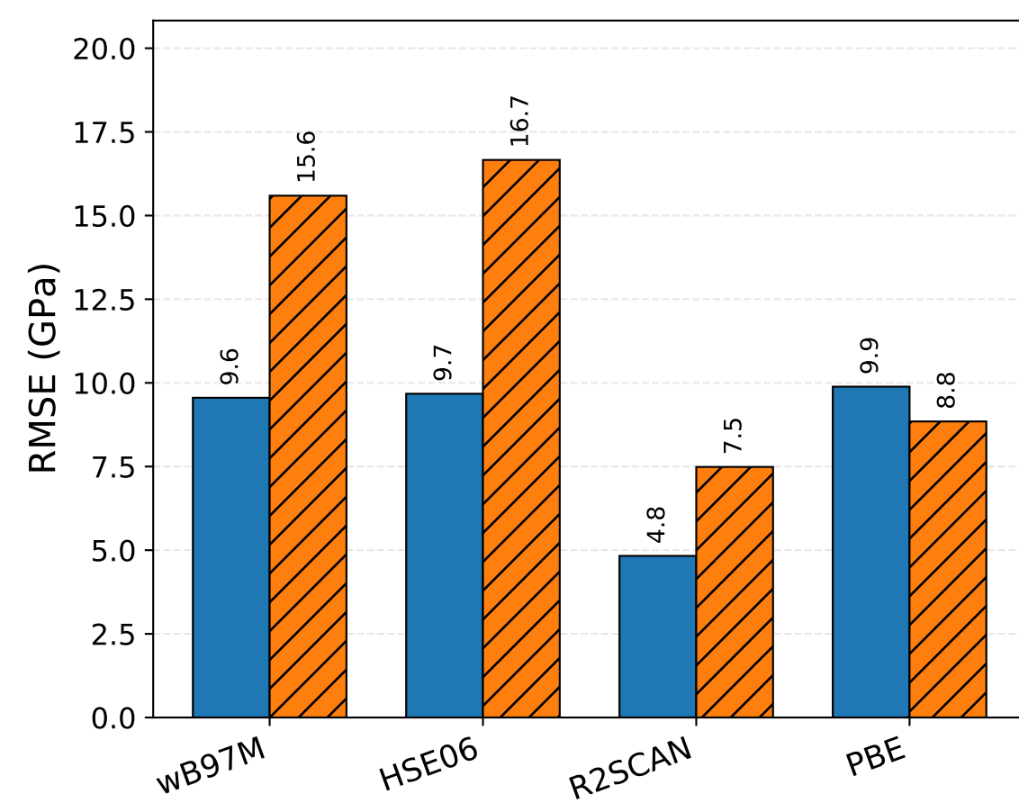
(c) Bulk modulus
