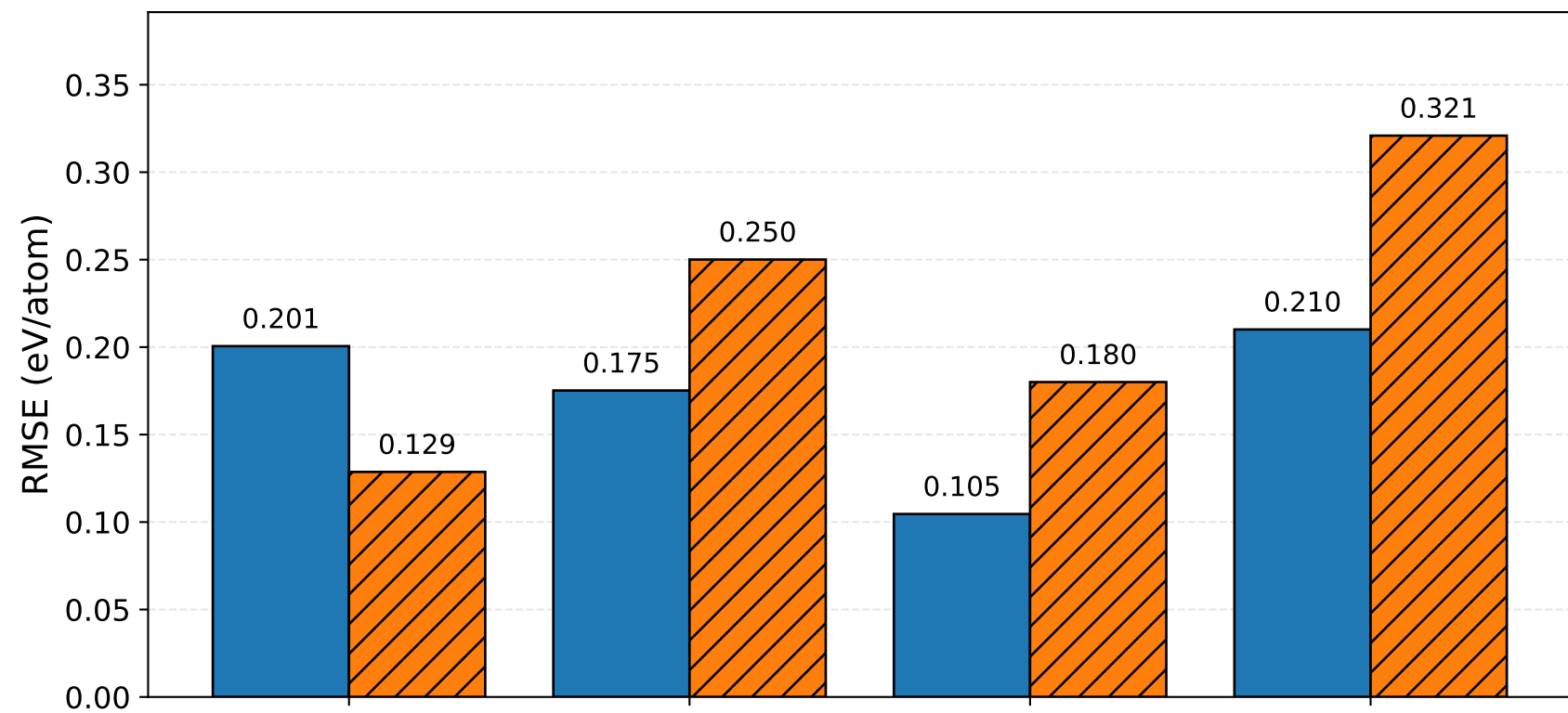
Cohesive energy
