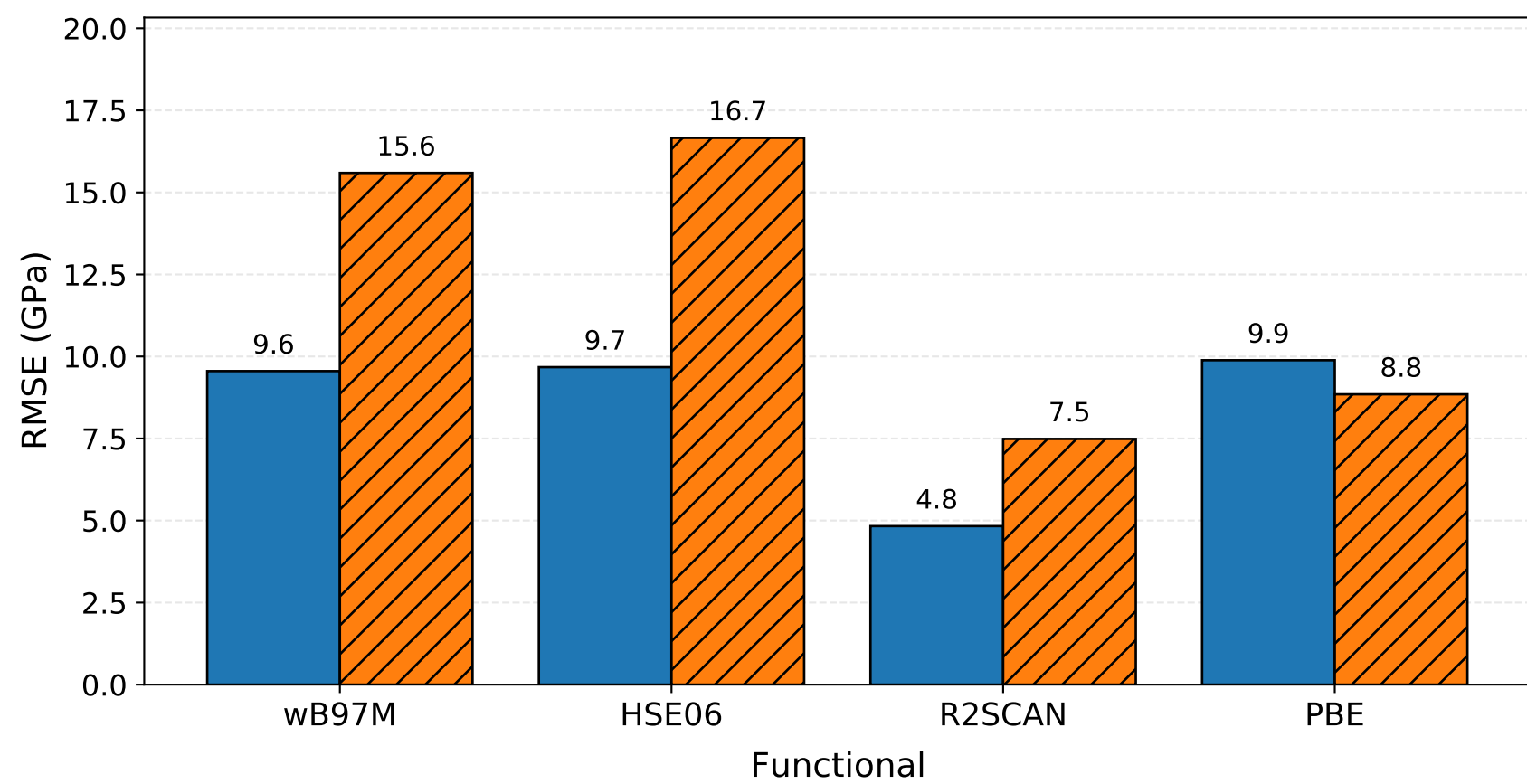
Bulk modulus
