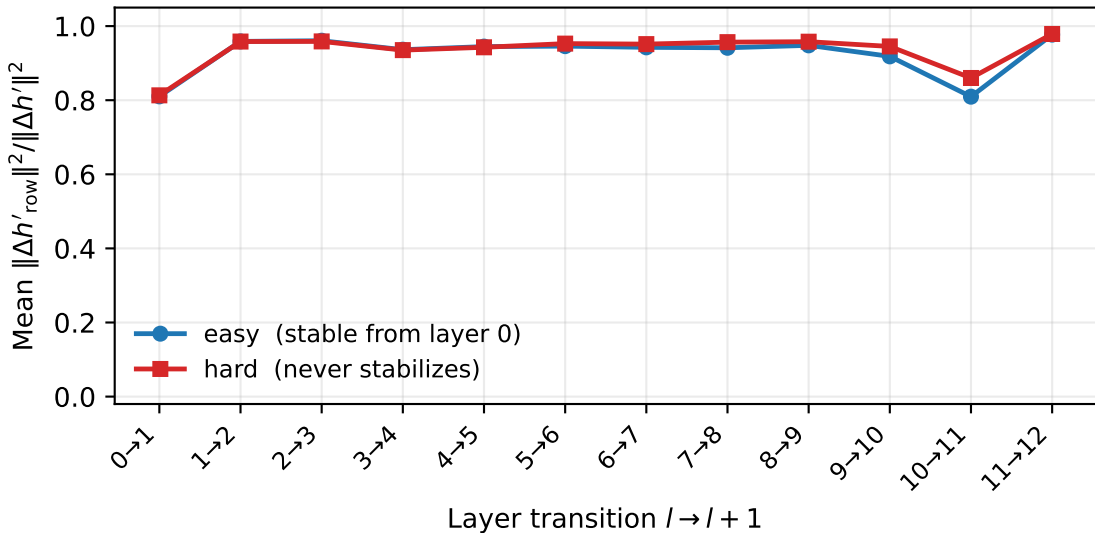
Fraction of \Delta h'_l in row( W_U ) (14,353 tokens per bucket, rank W_U = 753 )
