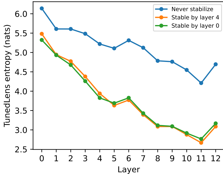
Prediction entropy by layer
