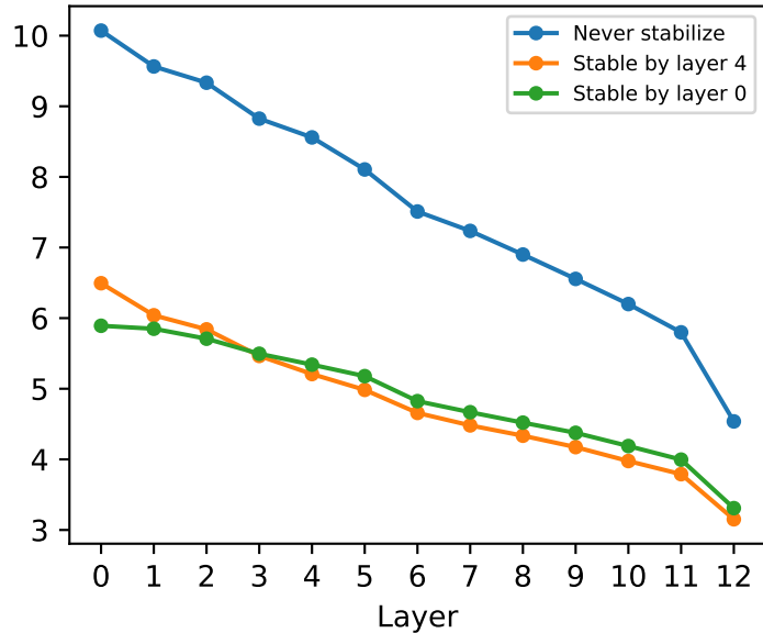
Cross-entropy by layer
