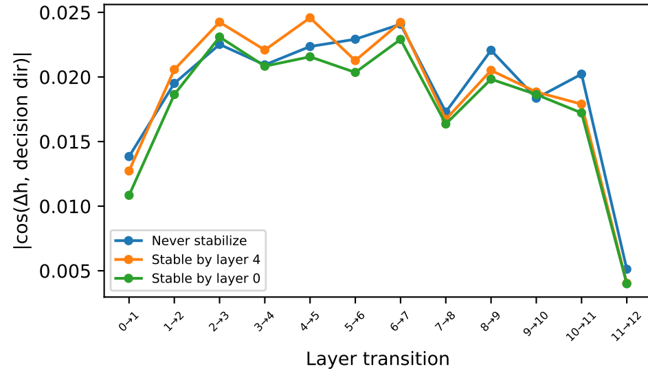
H3: Alignment of \Delta h with top1-top2 decision direction
