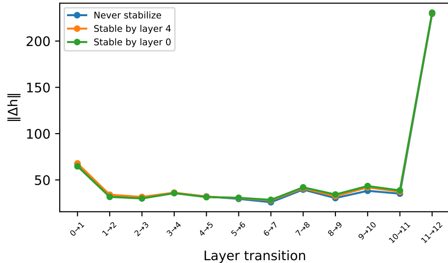
Magnitude of hidden state change (translated states)
