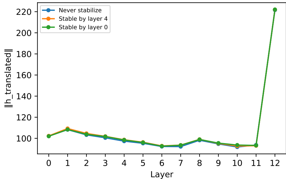
Translated hidden state norm by layer
