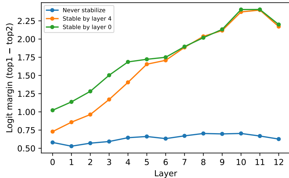
H1: Logit margin by layer
