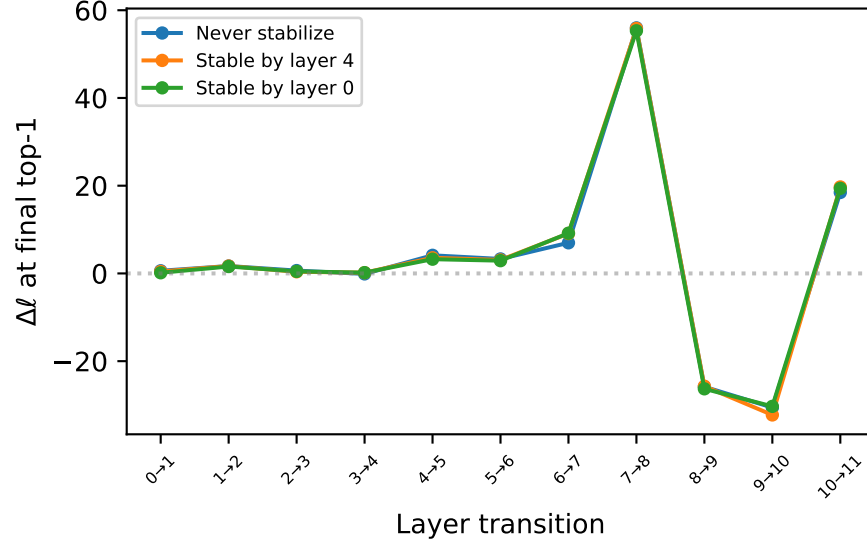
Logit update at eventual prediction (excl. 11→12)
