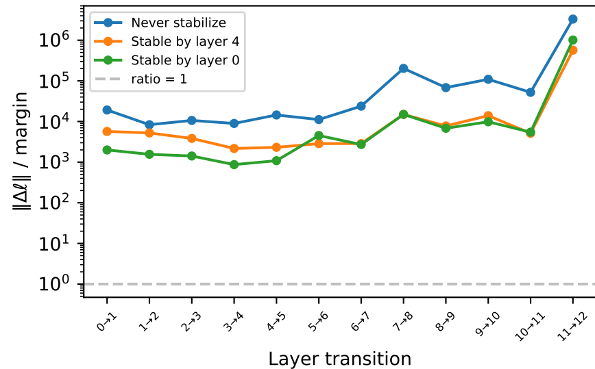
Logit update / margin ratio
