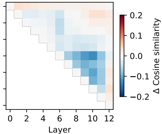
Difference (Low CE - High CE)
