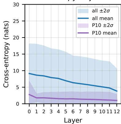
b) Cross-entropy trajectories
