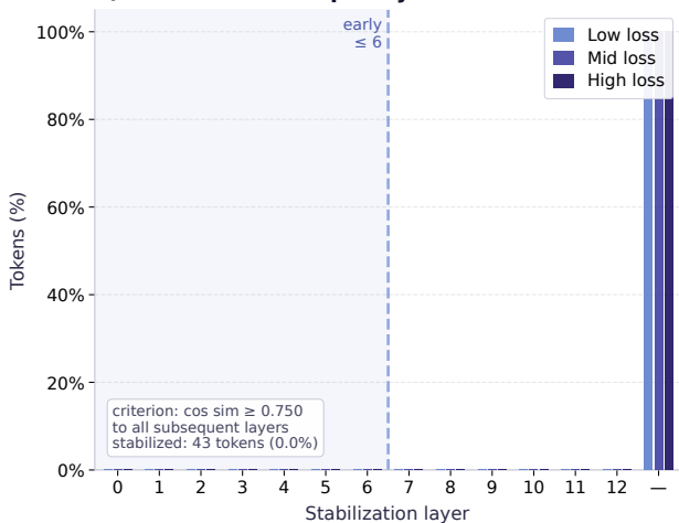
a) Stabilization depth by loss tier
