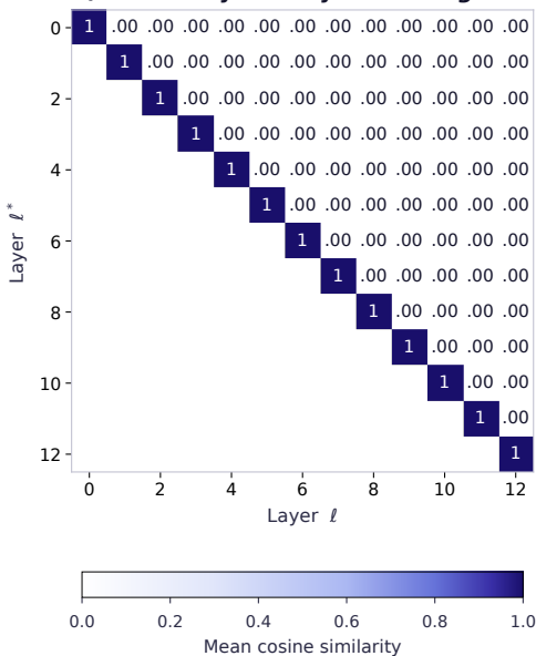
b) Similarity — early-stabilizing tokens ( \leq layer 6)
