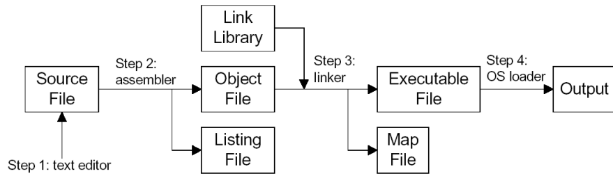
Figure 3–1 Assemble-Link-Execute Cycle.
