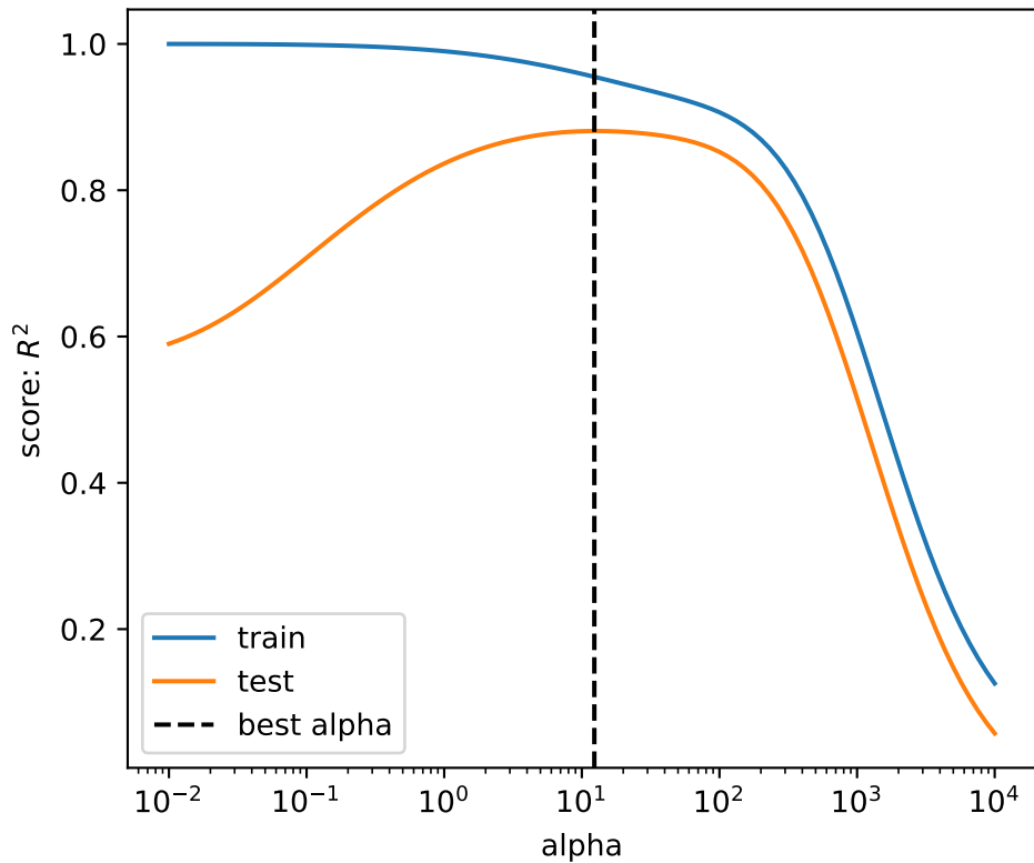
Validation curve for ridge
