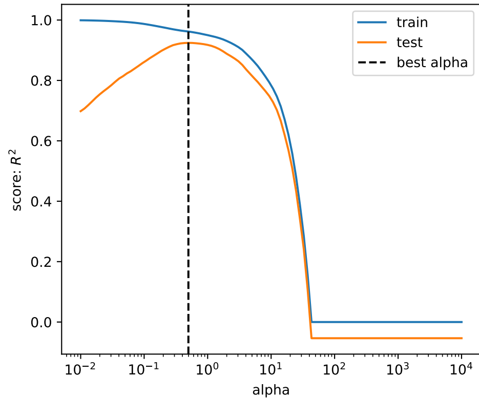
Validation curve for lasso
