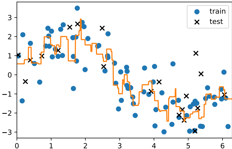
KNN Regression, K = 3
