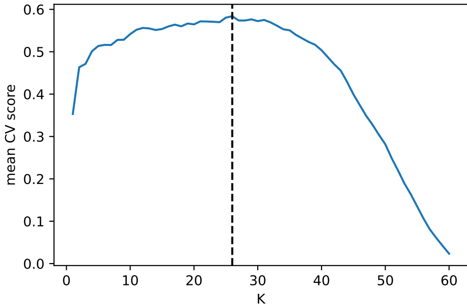
Cross-validation: best K = 26
