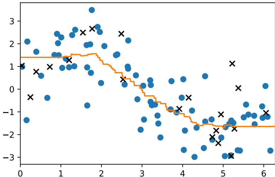
KNN Regression with Cross-Validated K
