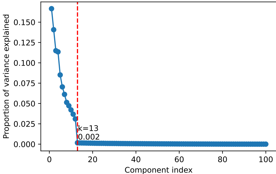
Scree Plot (Variance Ratio)
