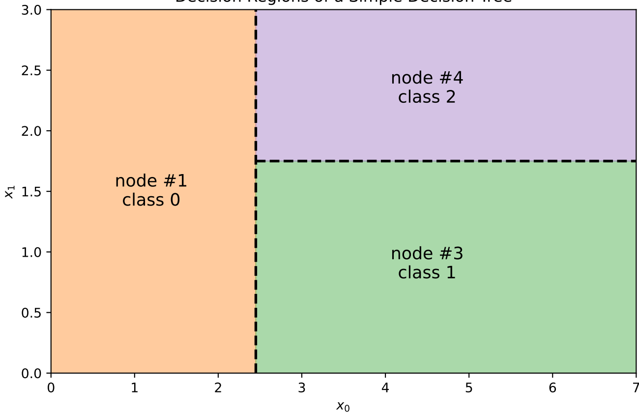
Decision Regions of a Simple Decision Tree
