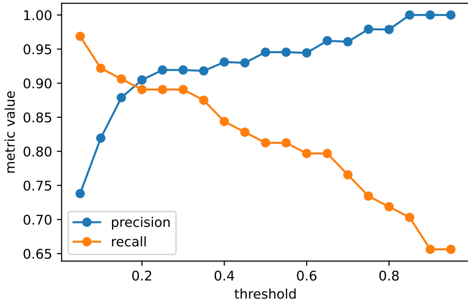
Precision and Recall versus Threshold
