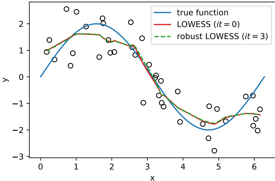
Ordinary versus Robust LOWESS
