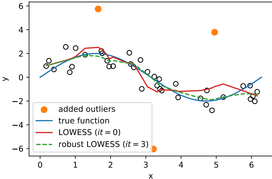
Ordinary versus Robust LOWESS with Outliers
