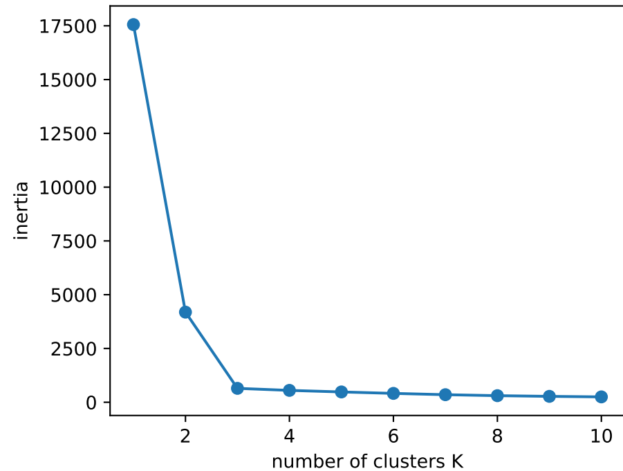
Elbow Plot
