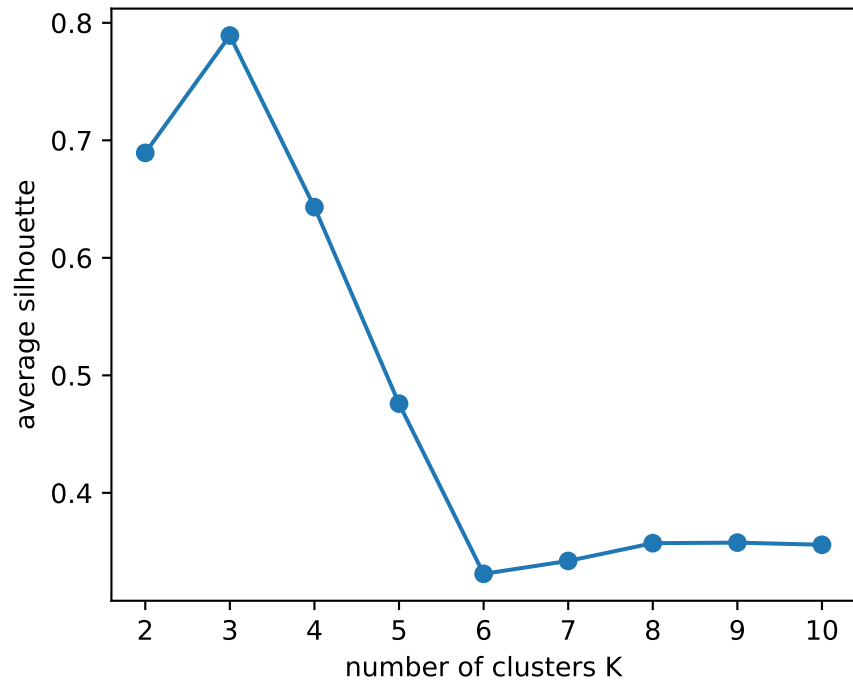
Silhouette Score
