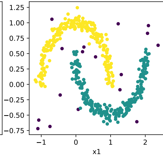
DBSCAN ARI = 0.94
