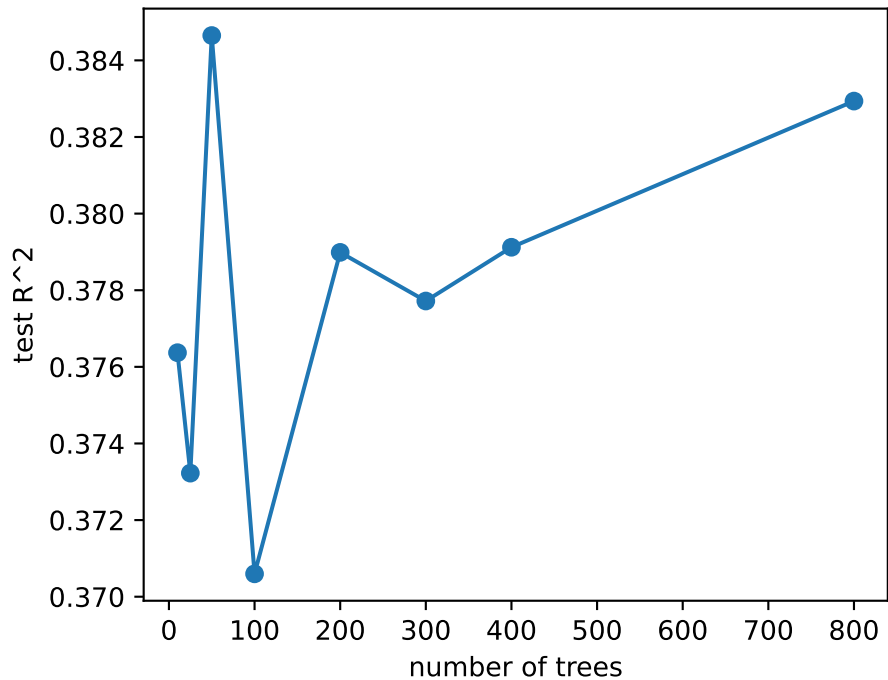
Validation score (using test set)
