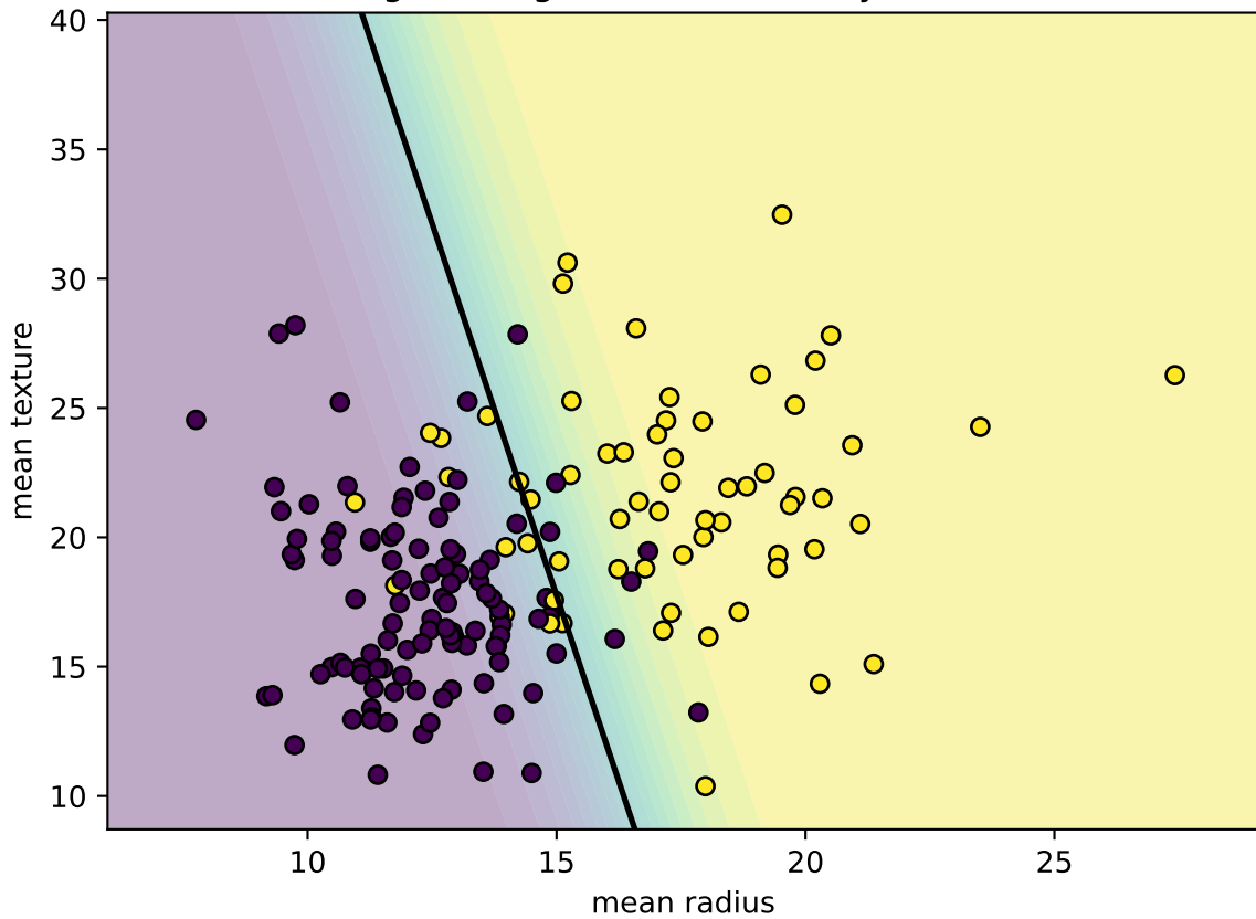
Logistic Regression Probability Surface
