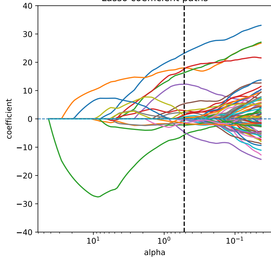
Lasso coefficient paths
