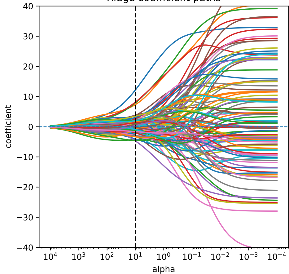
Ridge coefficient paths
