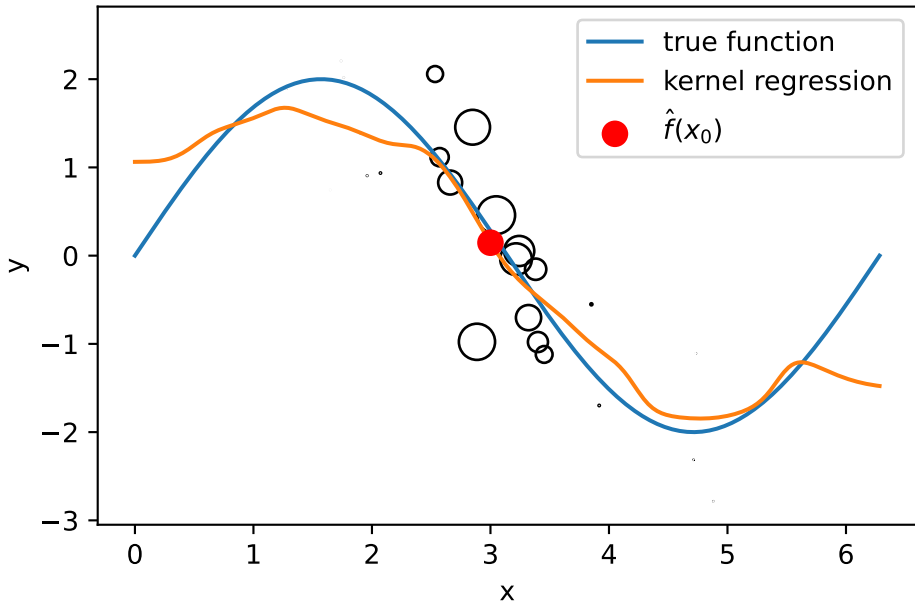
Kernel Weights Around a Target Point
