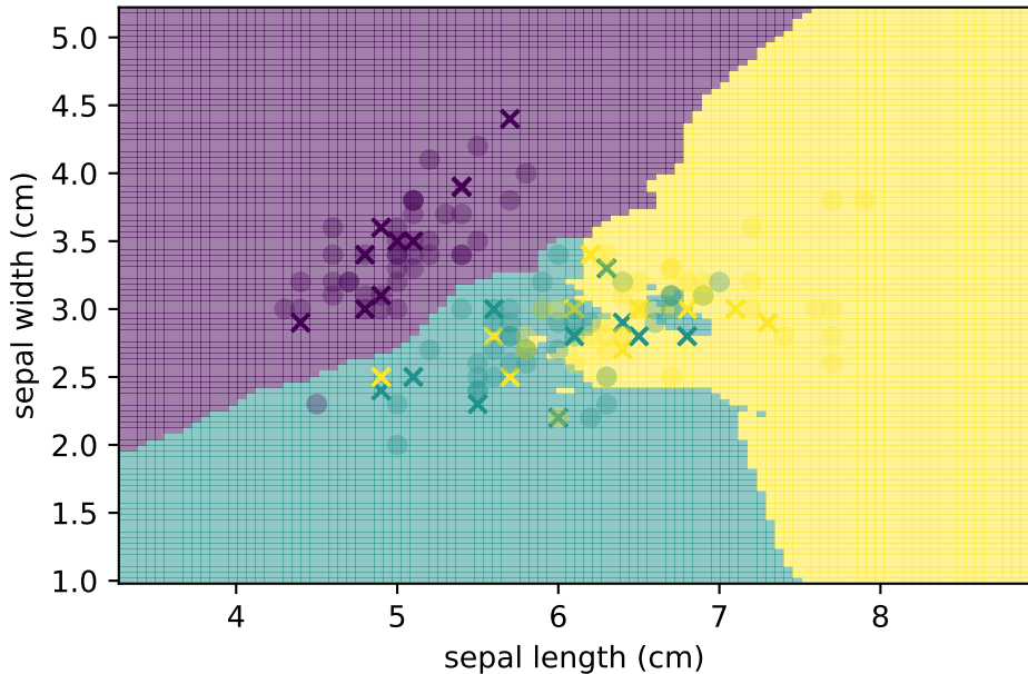
KNN Decision Boundary
