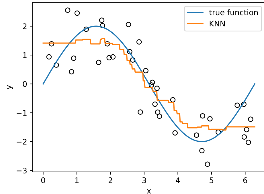
KNN Regression
