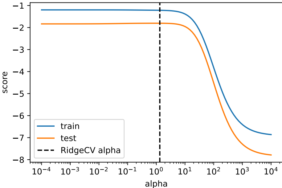
Validation curve for ridge regression
