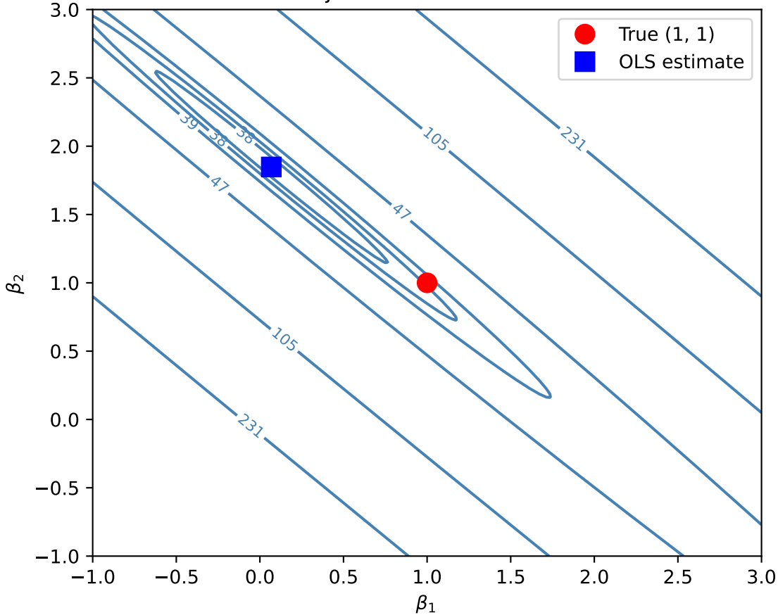
OLS Objective Function Contours
