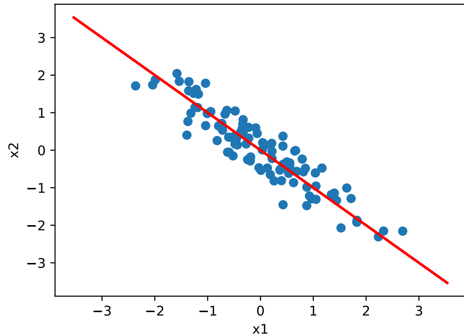
Centered + Scaled
