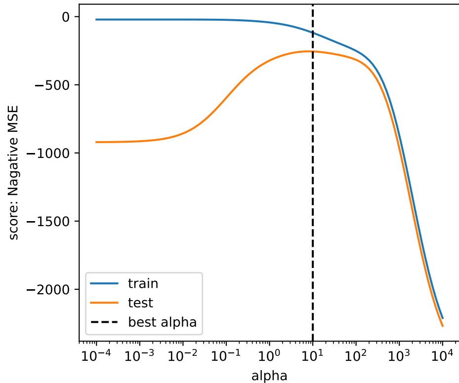
Validation curve for ridge
