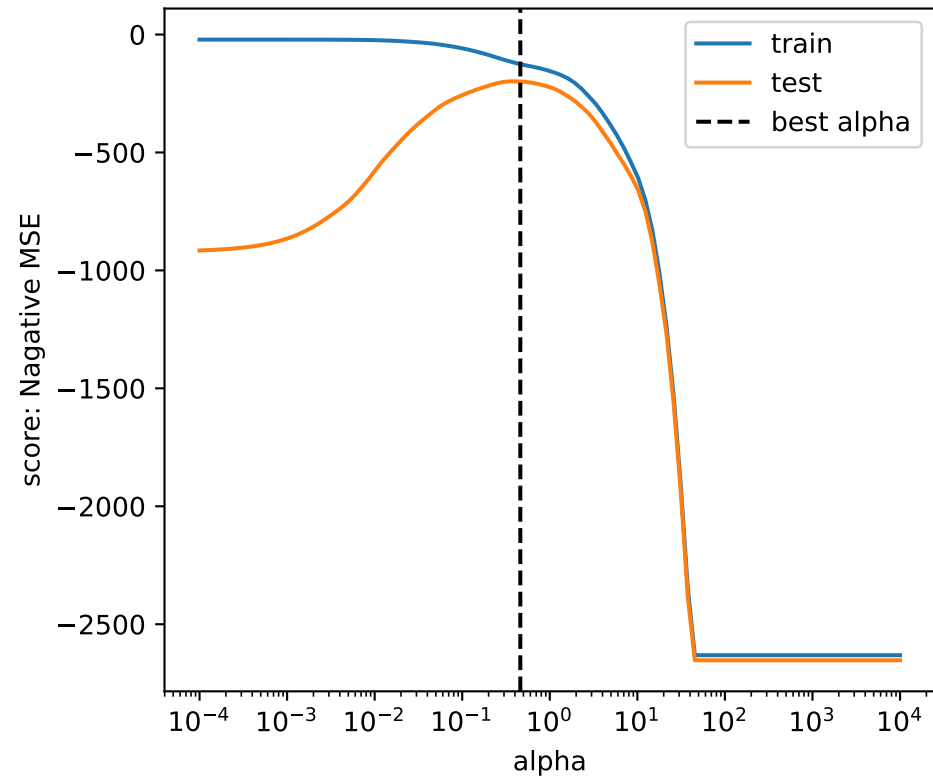
Validation curve for lasso
