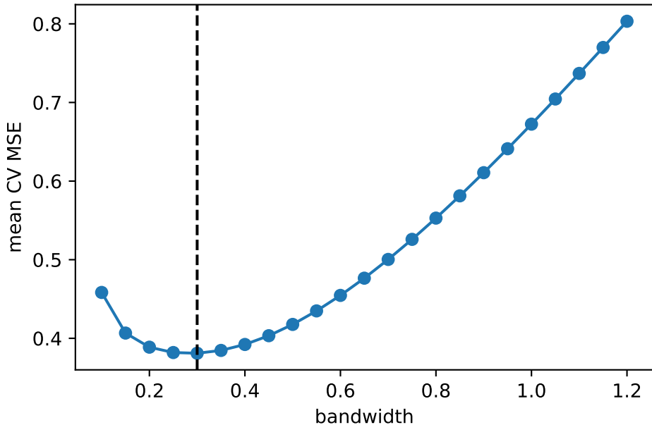
Bandwidth Selection by Cross-Validation
