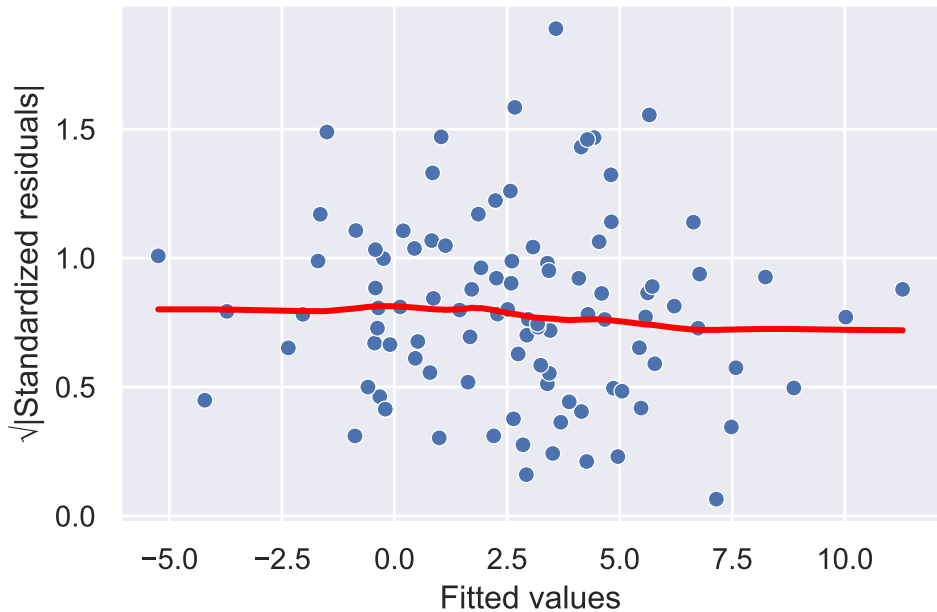
Scale-Location
