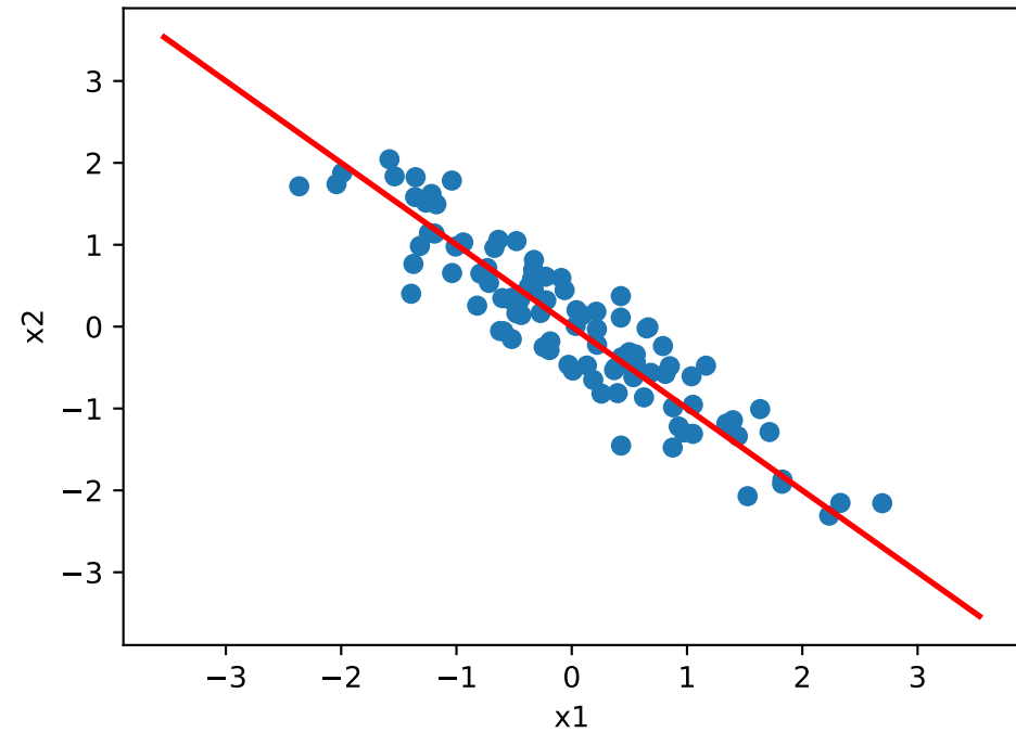
Centered + Scaled
