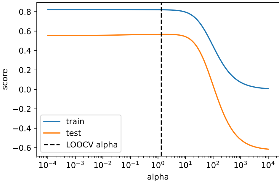
Validation curve for ridge regression
