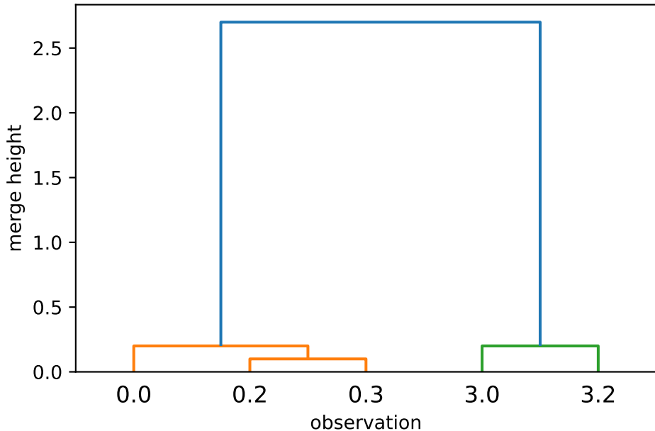
Dendrogram for Five Points
